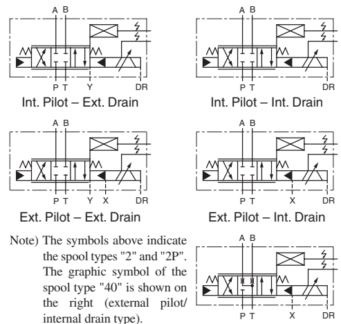
Graphic Symbols
