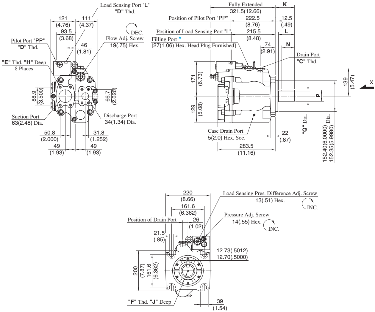
View Arrow X
