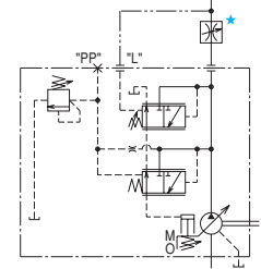
Graphic Symbol
